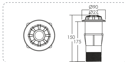
Outlet Fitting (Concrete Pool)
